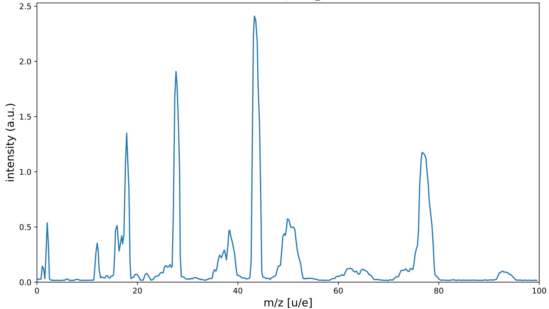
QMS-TPD: Mass spectra_Benzen.txt
